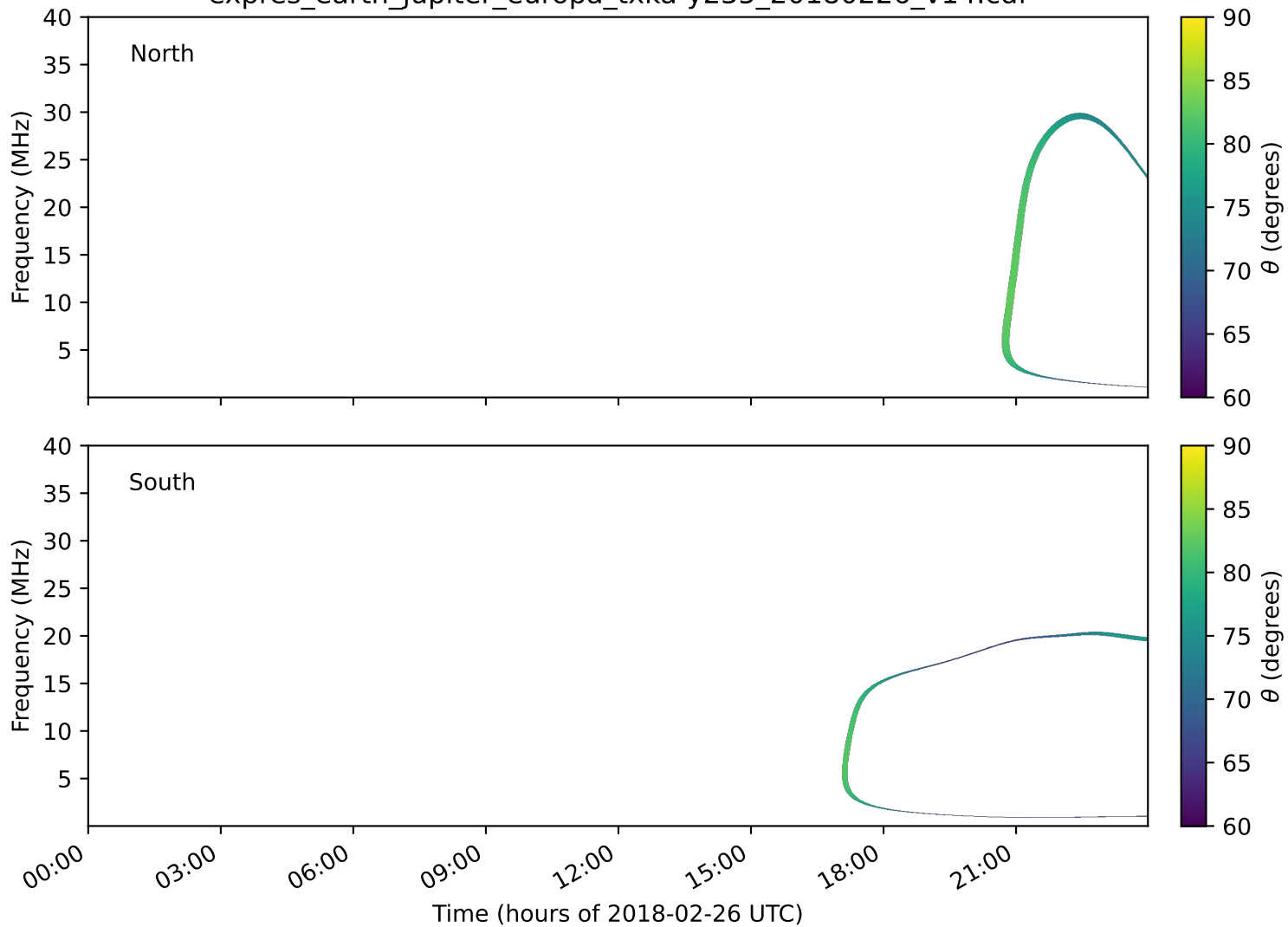
expres_earth_jupiter_europa_txka-y235_20180226_v14.cdf
