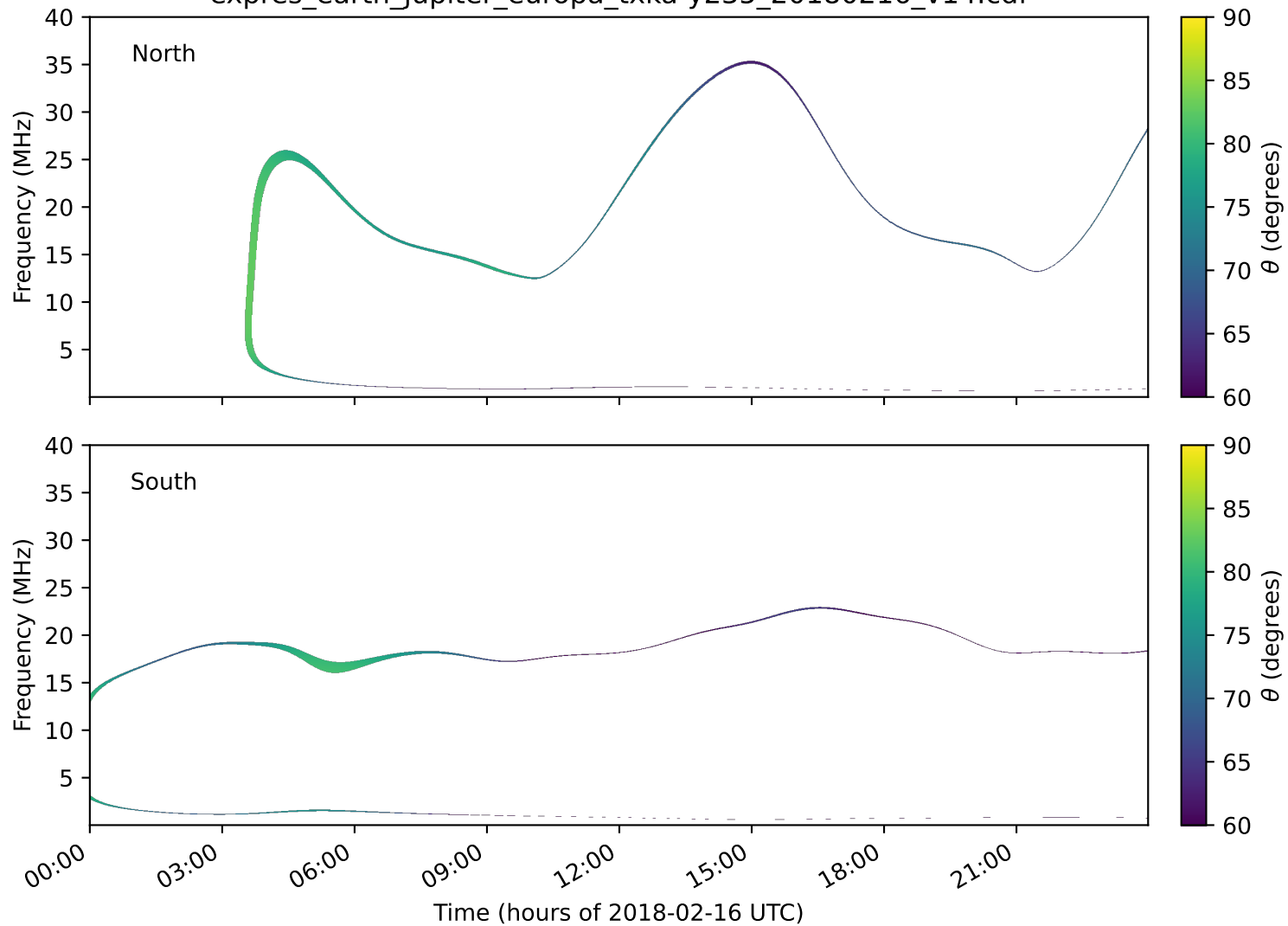
expres_earth_jupiter_europa_txka-y235_20180216_v14.cdf
