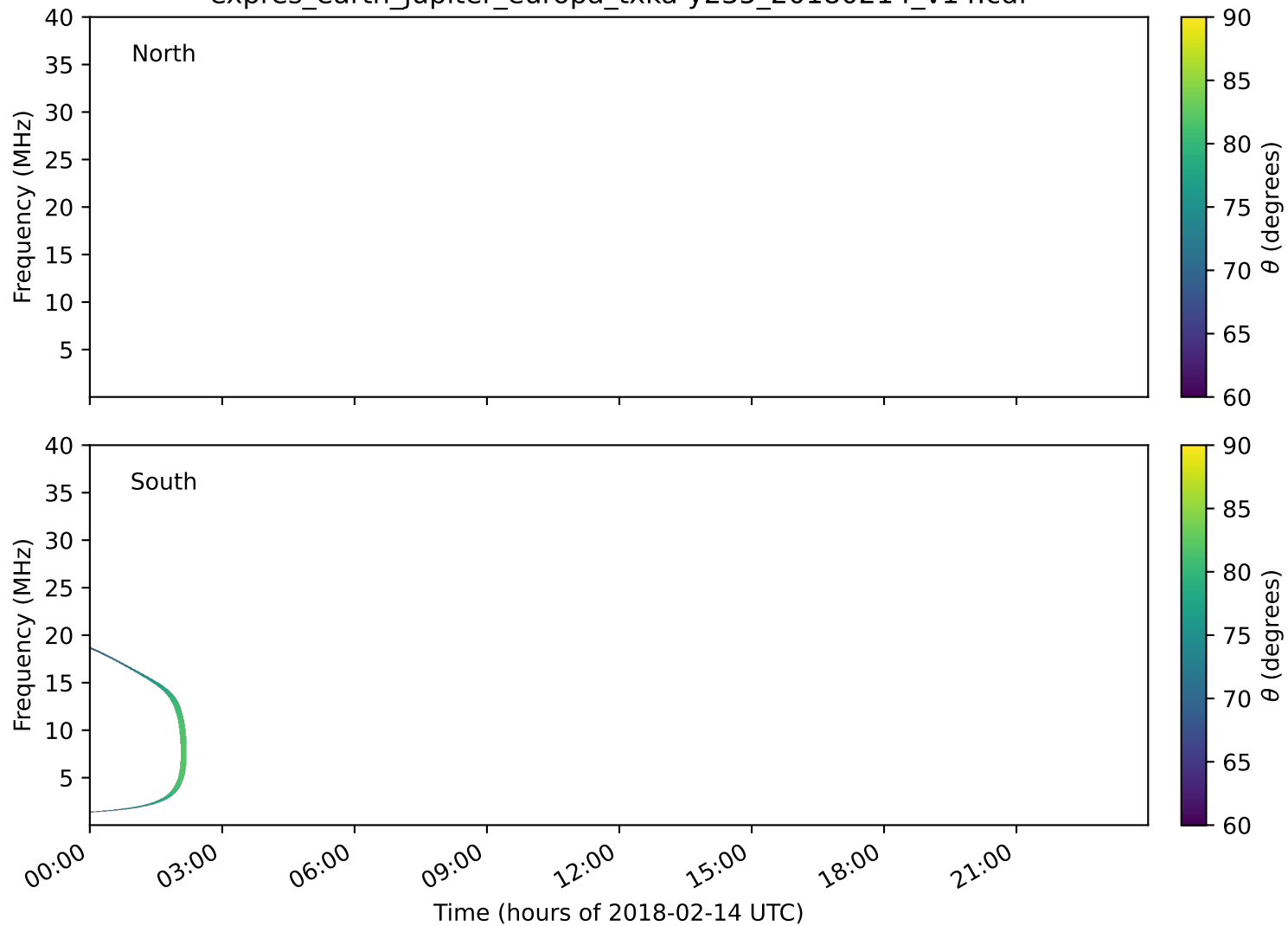
expres_earth_jupiter_europa_txka-y235_20180214_v14.cdf
