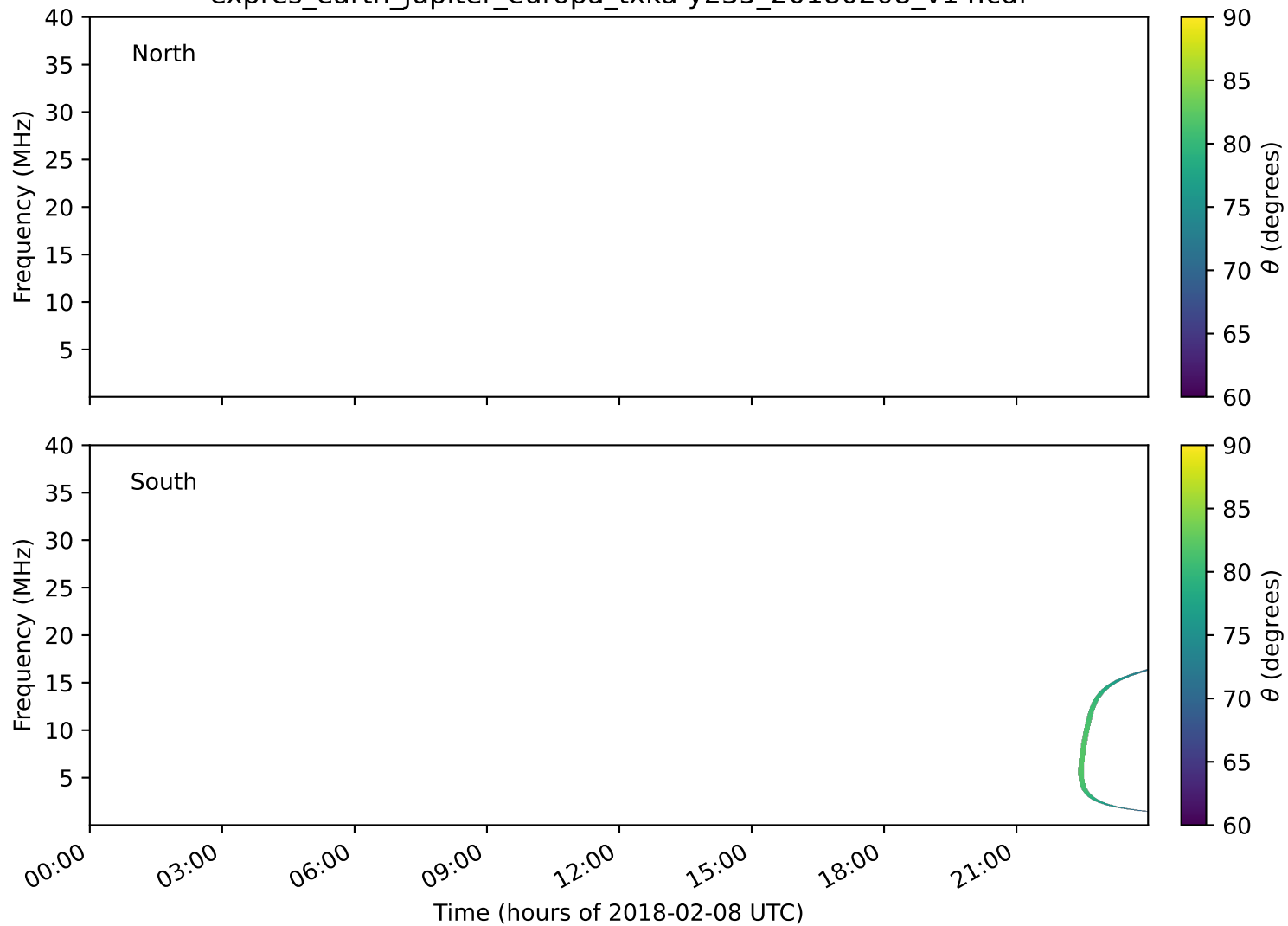
expres_earth_jupiter_europa_txka-y235_20180208_v14.cdf
