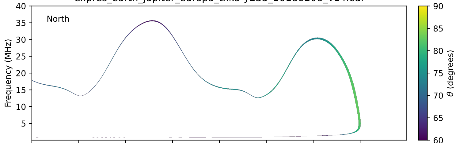
expres_earth_jupiter_europa_txka-y235_20180206_v14.cdf
