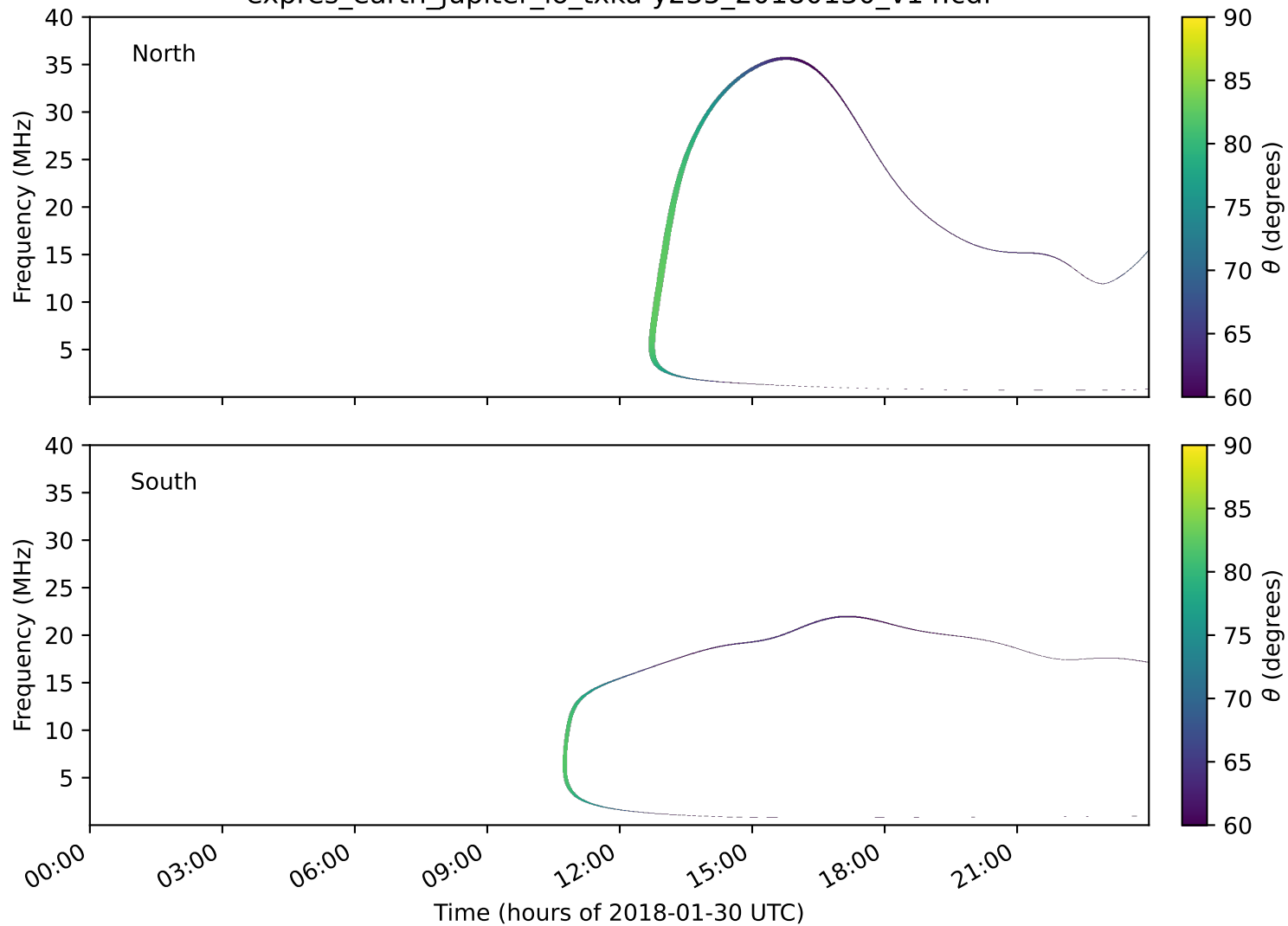
expres_earth_jupiter_io_txka-y235_20180130_v14.cdf
