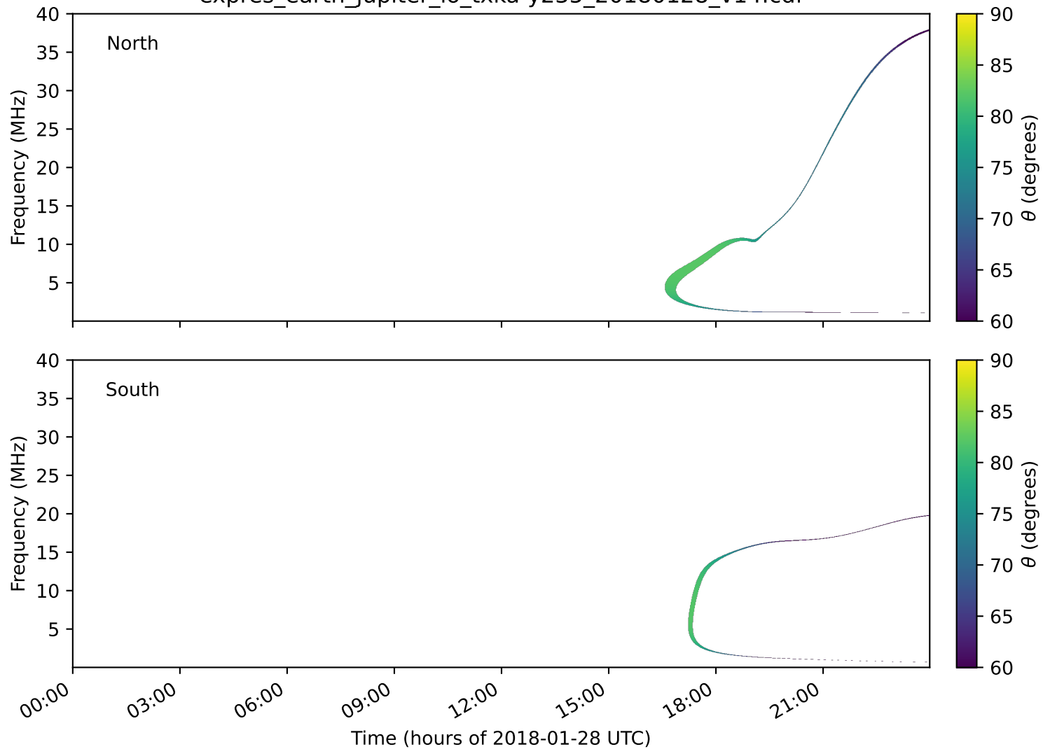
expres_earth_jupiter_io_txka-y235_20180128_v14.cdf
