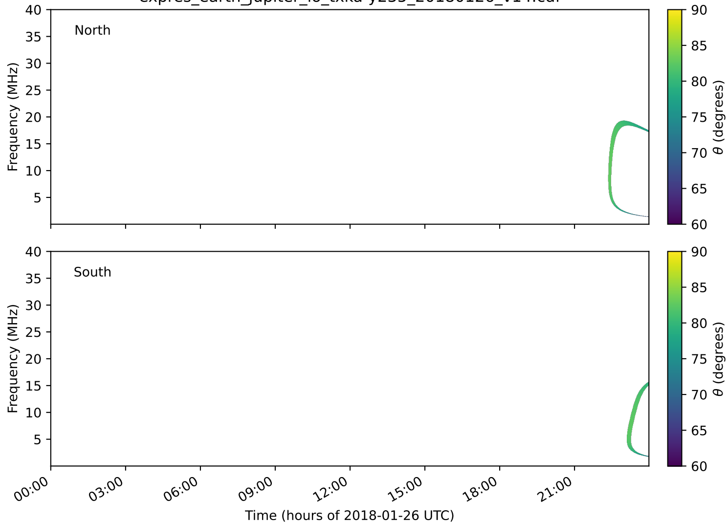
expres_earth_jupiter_io_txka-y235_20180126_v14.cdf
