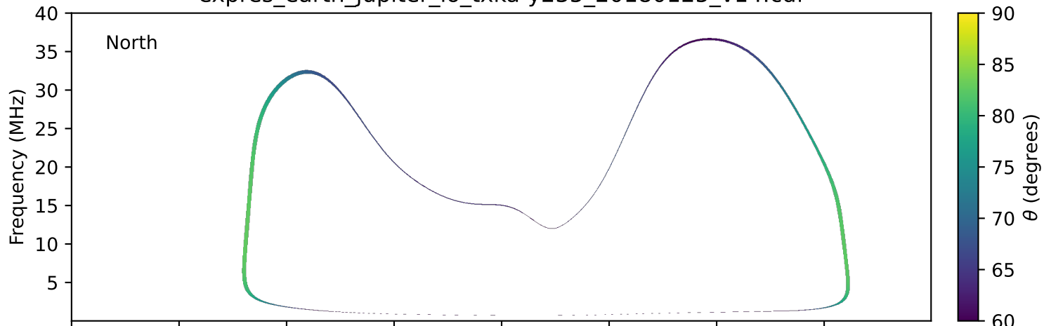
expres_earth_jupiter_io_txka-y235_20180125_v14.cdf
