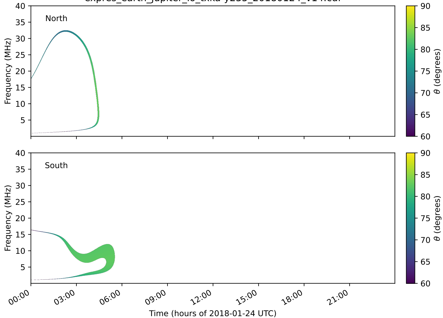
expres_earth_jupiter_io_txka-y235_20180124_v14.cdf
