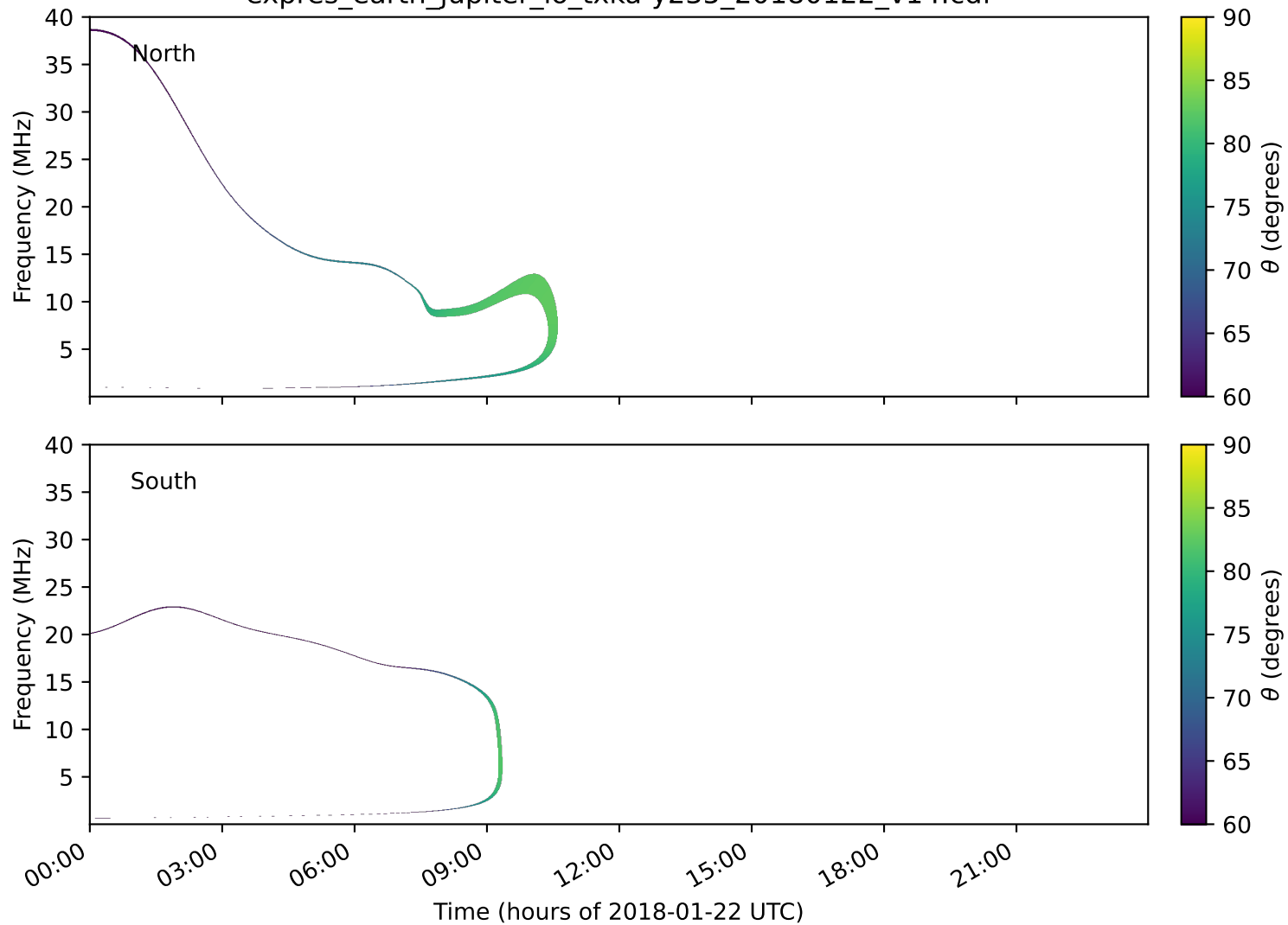
expres_earth_jupiter_io_txka-y235_20180122_v14.cdf
