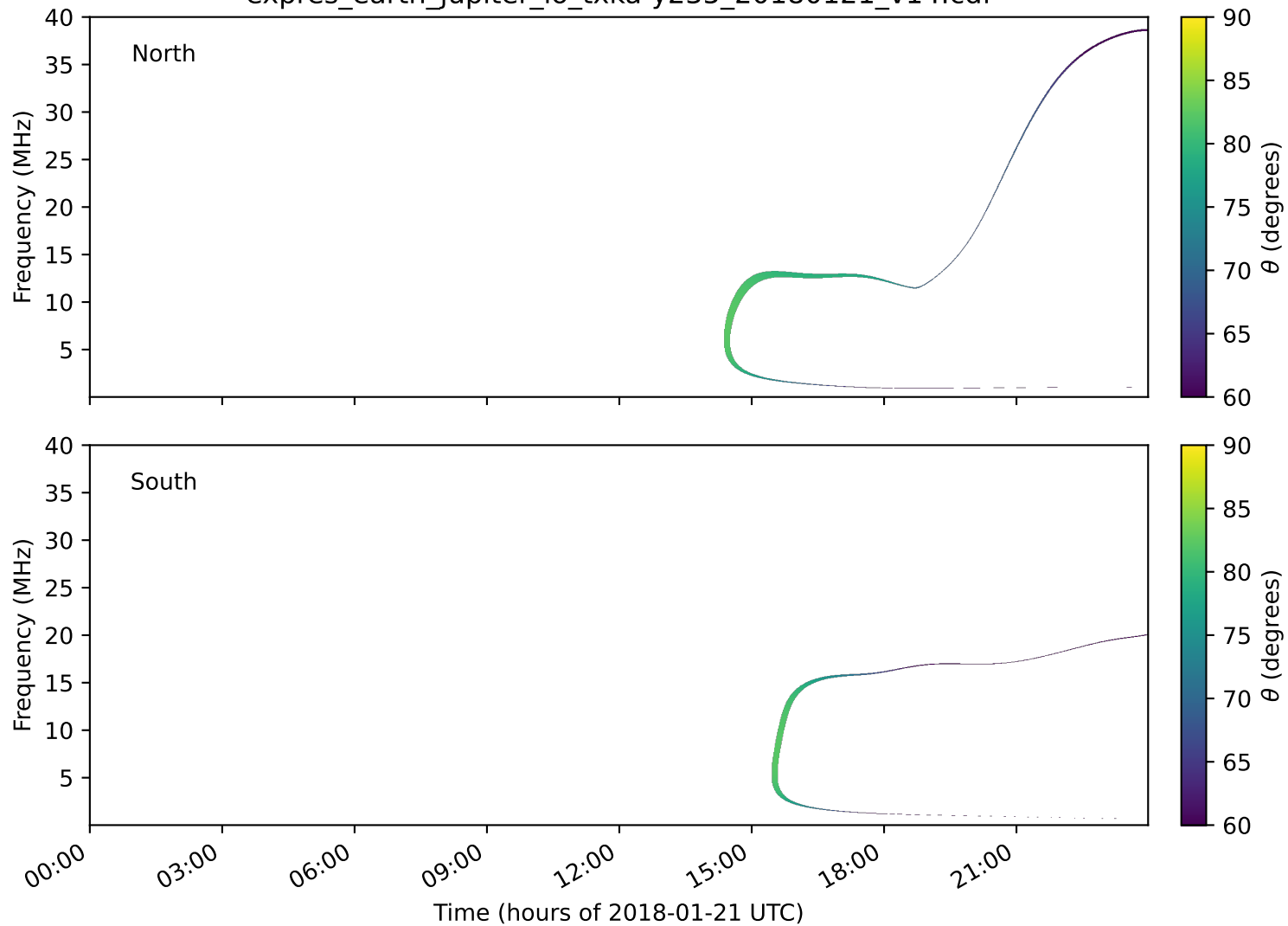
expres_earth_jupiter_io_txka-y235_20180121_v14.cdf
