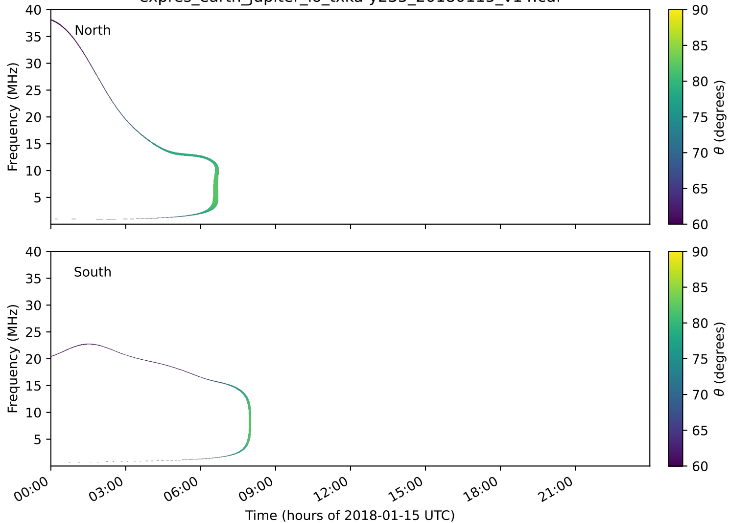
expres_earth_jupiter_io_txka-y235_20180115_v14.cdf
