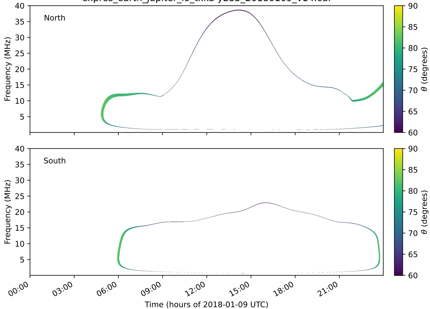
expres_earth_jupiter_io_txka-y235_20180109_v14.cdf
