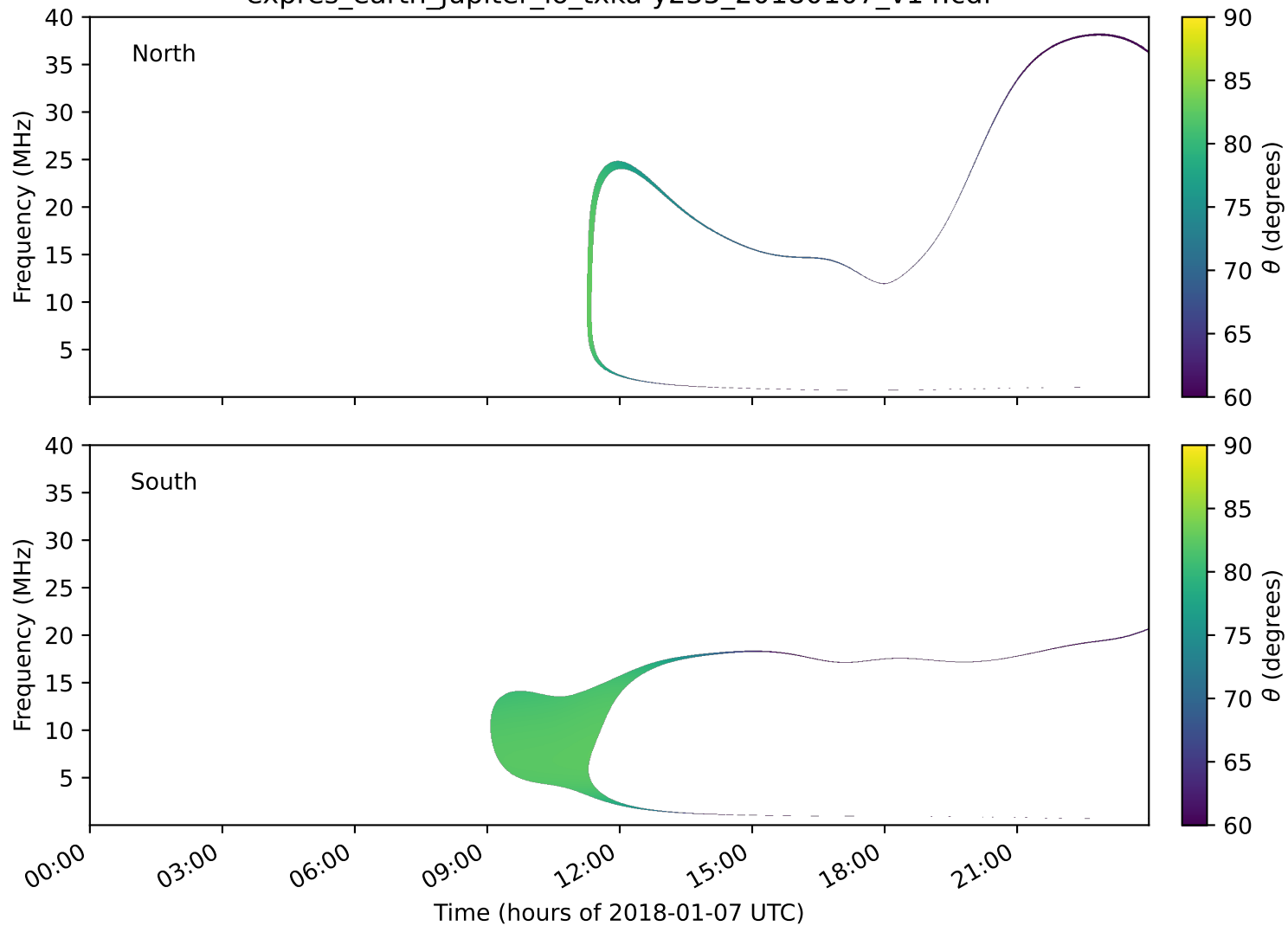
expres_earth_jupiter_io_txka-y235_20180107_v14.cdf
