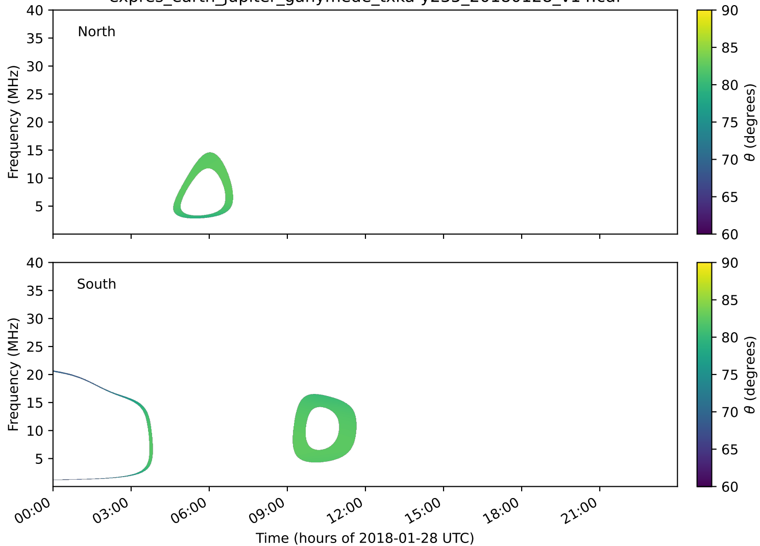
expres_earth_jupiter_ganymede_txka-y235_20180128_v14.cdf
