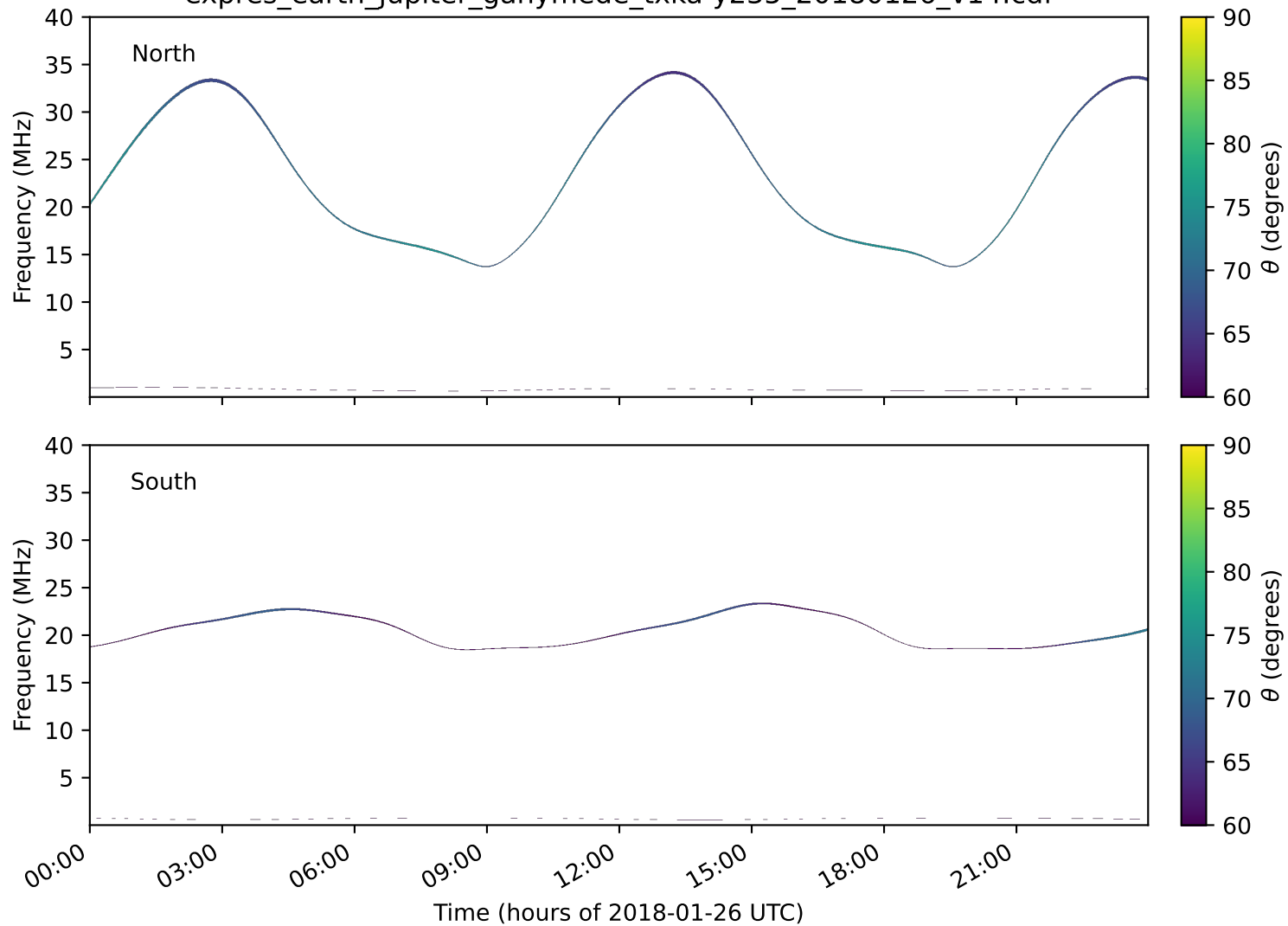
expres_earth_jupiter_ganymede_txka-y235_20180126_v14.cdf
