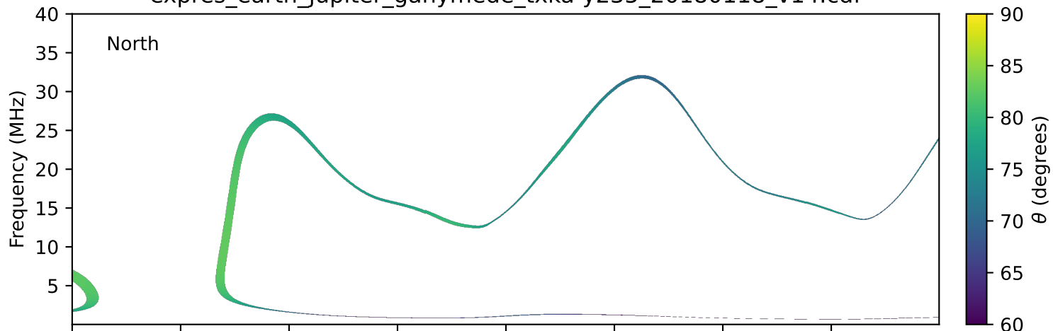
expres_earth_jupiter_ganymede_txka-y235_20180118_v14.cdf
