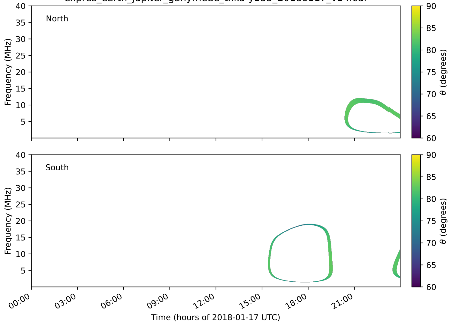
expres_earth_jupiter_ganymede_txka-y235_20180117_v14.cdf
