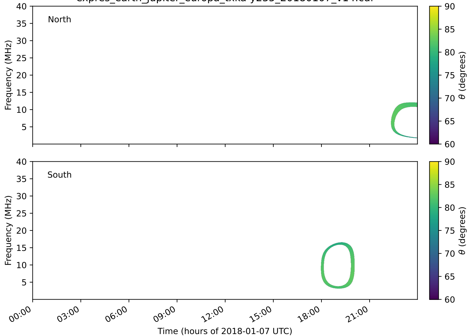
expres_earth_jupiter_europa_txka-y235_20180107_v14.cdf
