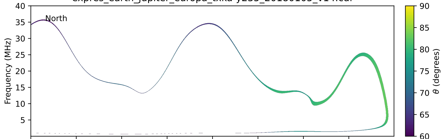
expres_earth_jupiter_europa_txka-y235_20180105_v14.cdf
