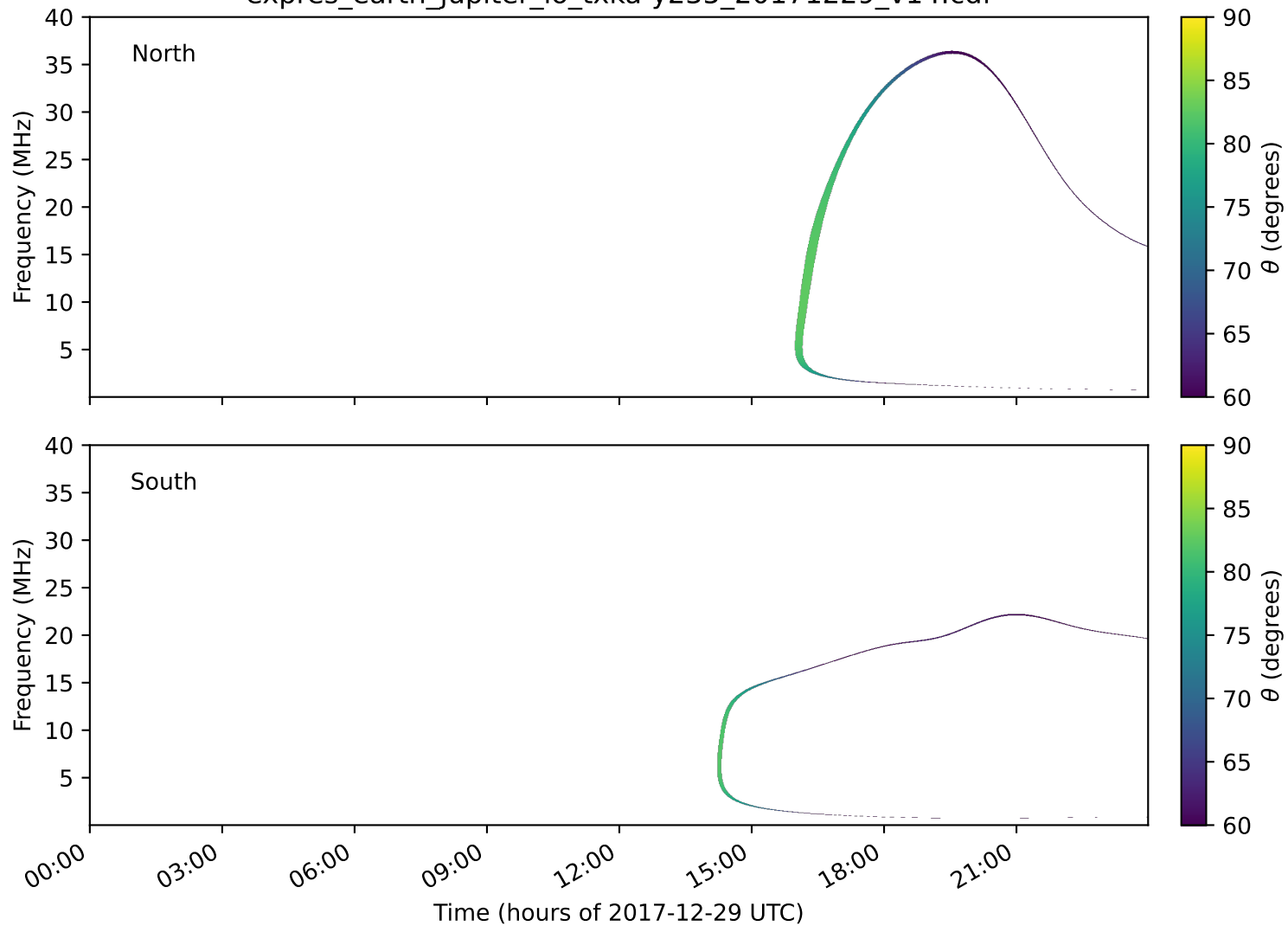
expres_earth_jupiter_io_txka-y235_20171229_v14.cdf
