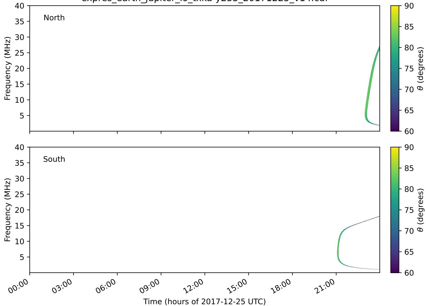
expres_earth_jupiter_io_txka-y235_20171225_v14.cdf
