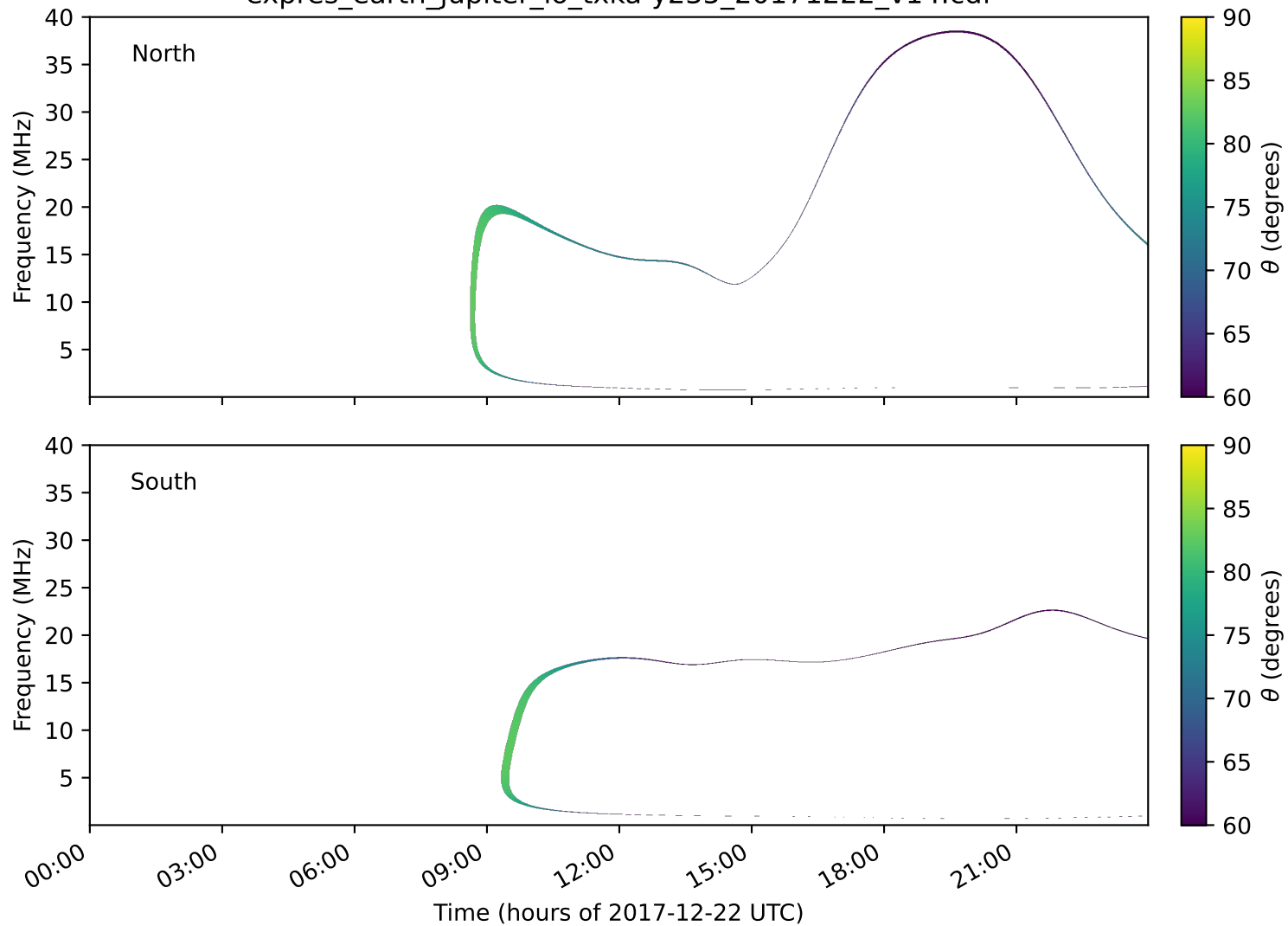
expres_earth_jupiter_io_txka-y235_20171222_v14.cdf
