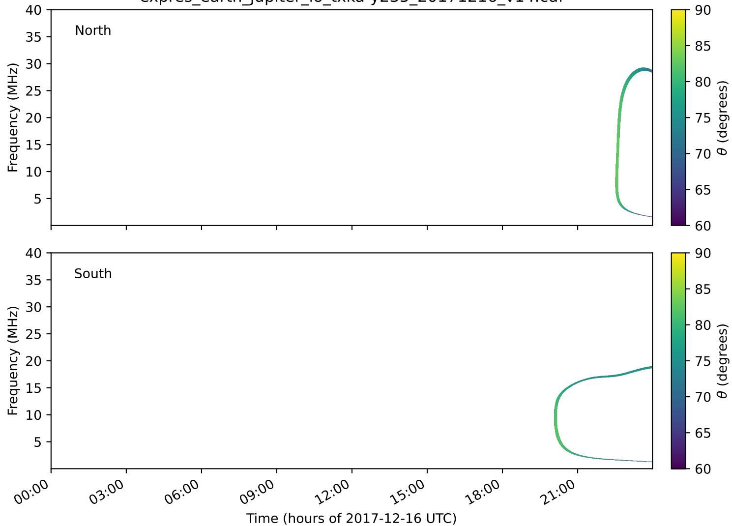
expres_earth_jupiter_io_txka-y235_20171216_v14.cdf
