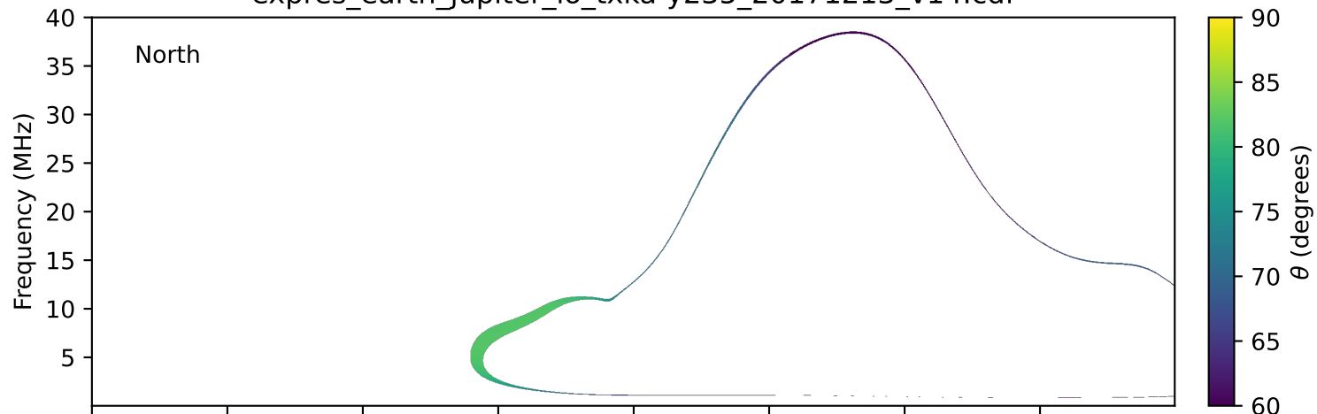
expres_earth_jupiter_io_txka-y235_20171213_v14.cdf
