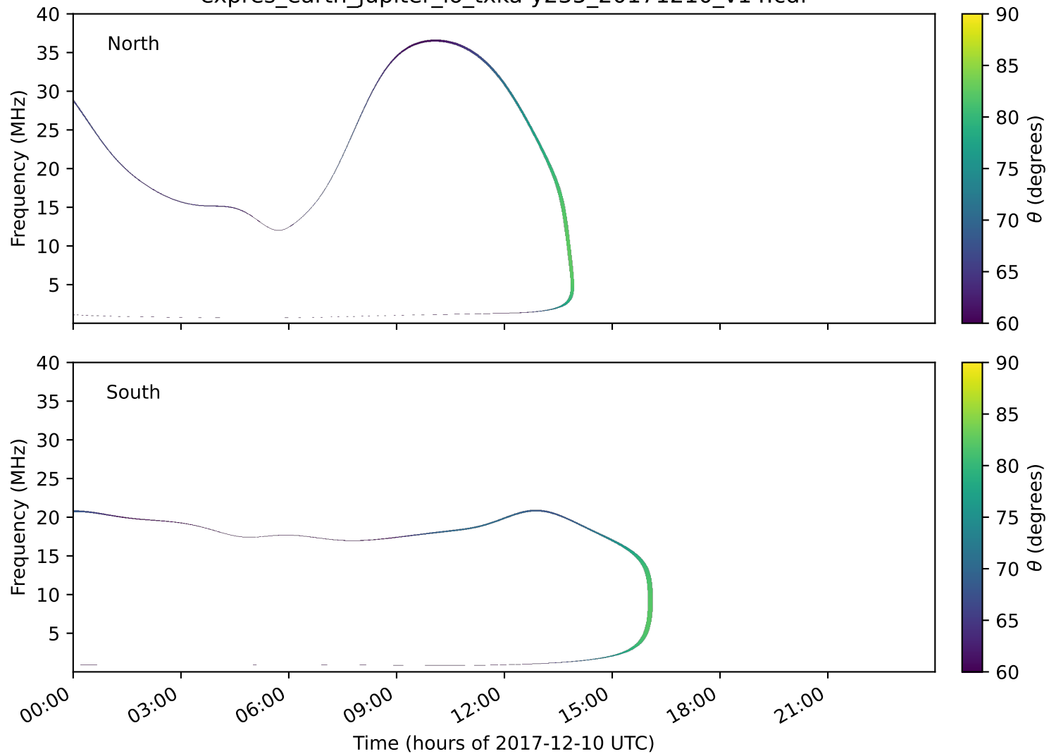
expres_earth_jupiter_io_txka-y235_20171210_v14.cdf
