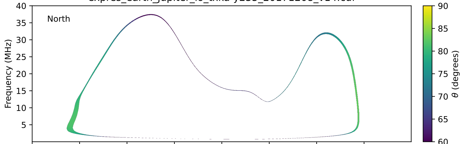
expres_earth_jupiter_io_txka-y235_20171208_v14.cdf
