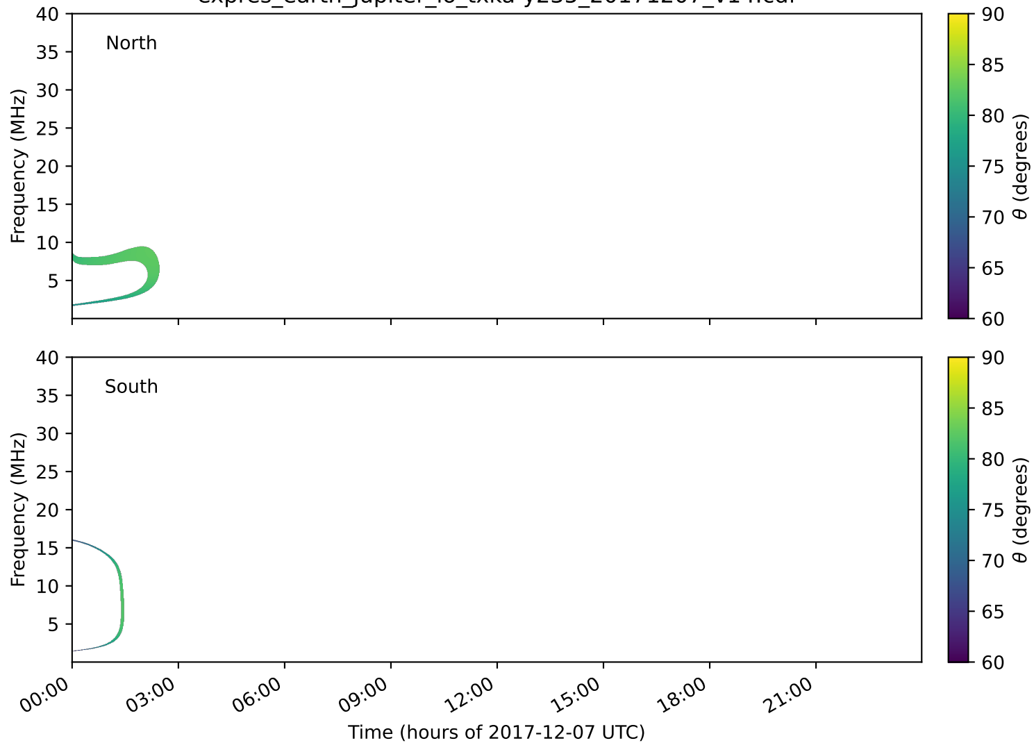
expres_earth_jupiter_io_txka-y235_20171207_v14.cdf
