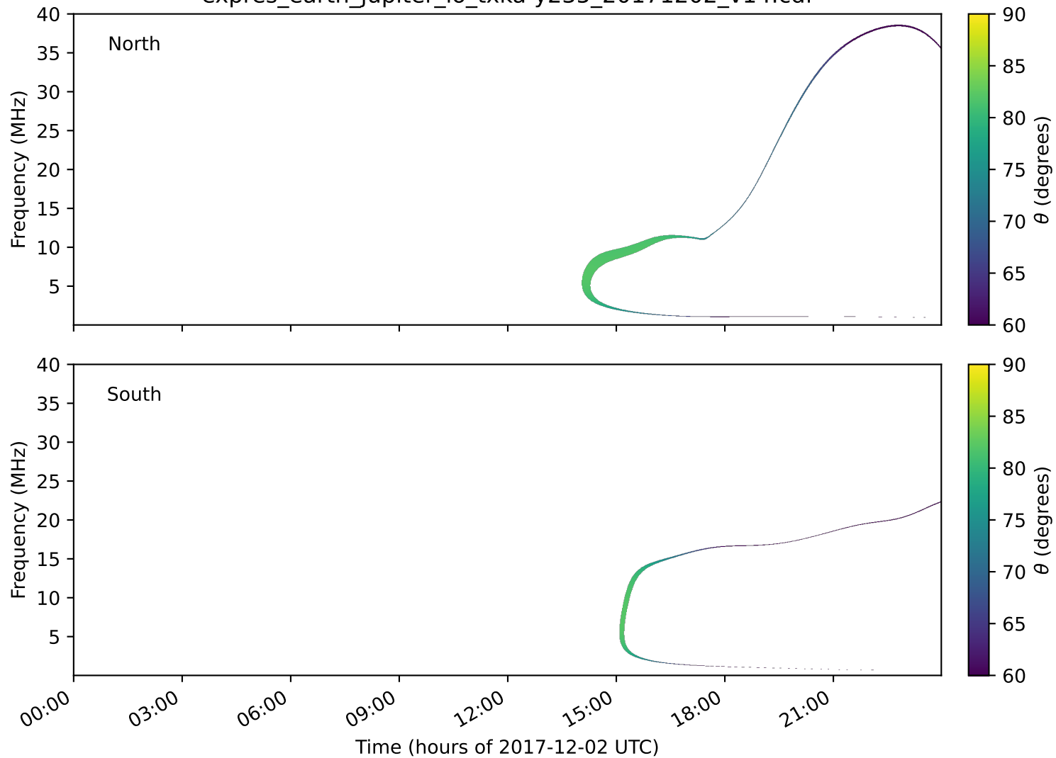
expres_earth_jupiter_io_txka-y235_20171202_v14.cdf
