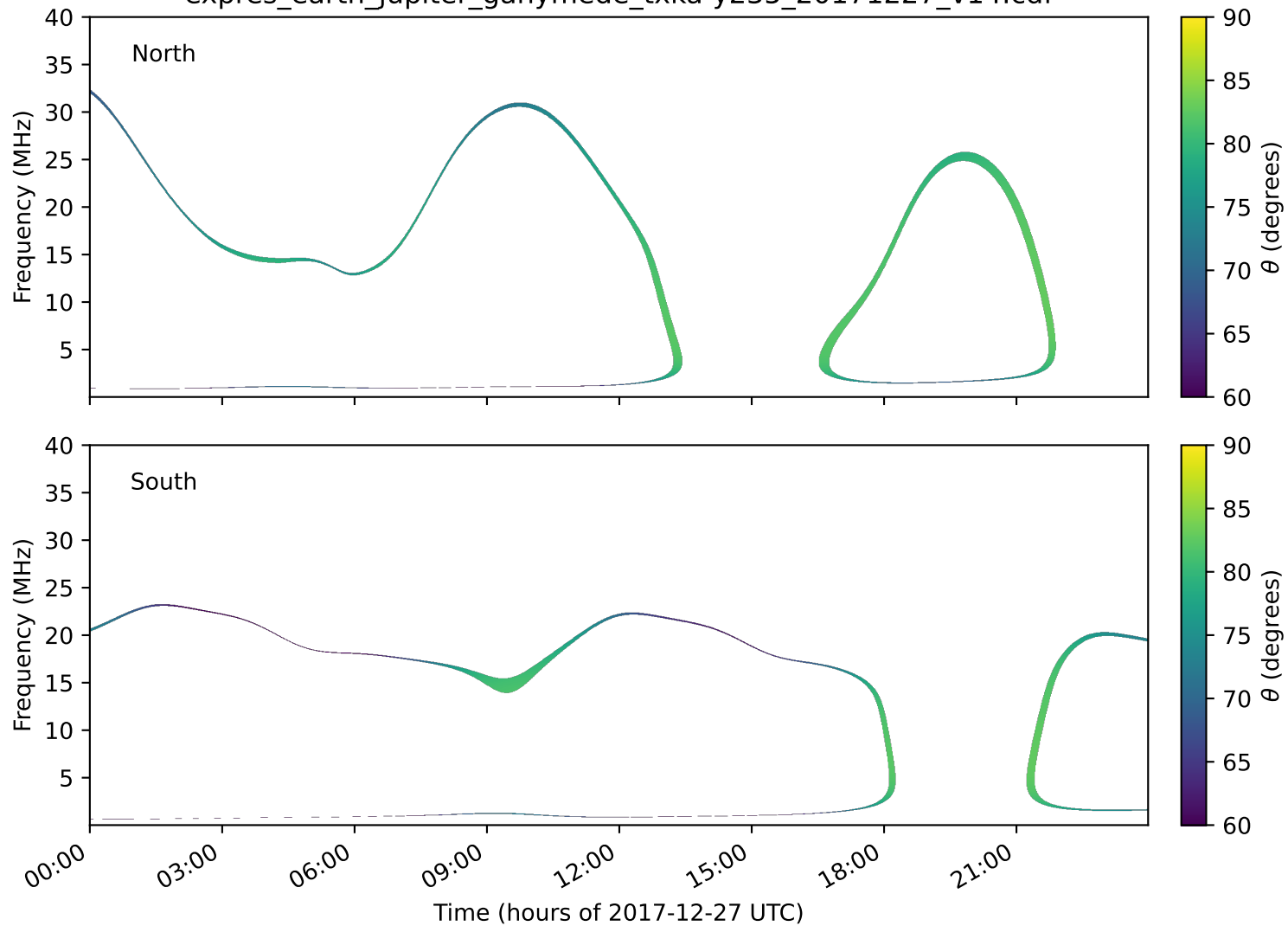
expres_earth_jupiter_ganymede_txka-y235_20171227_v14.cdf
