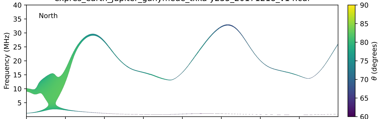
expres_earth_jupiter_ganymede_txka-y235_20171218_v14.cdf
