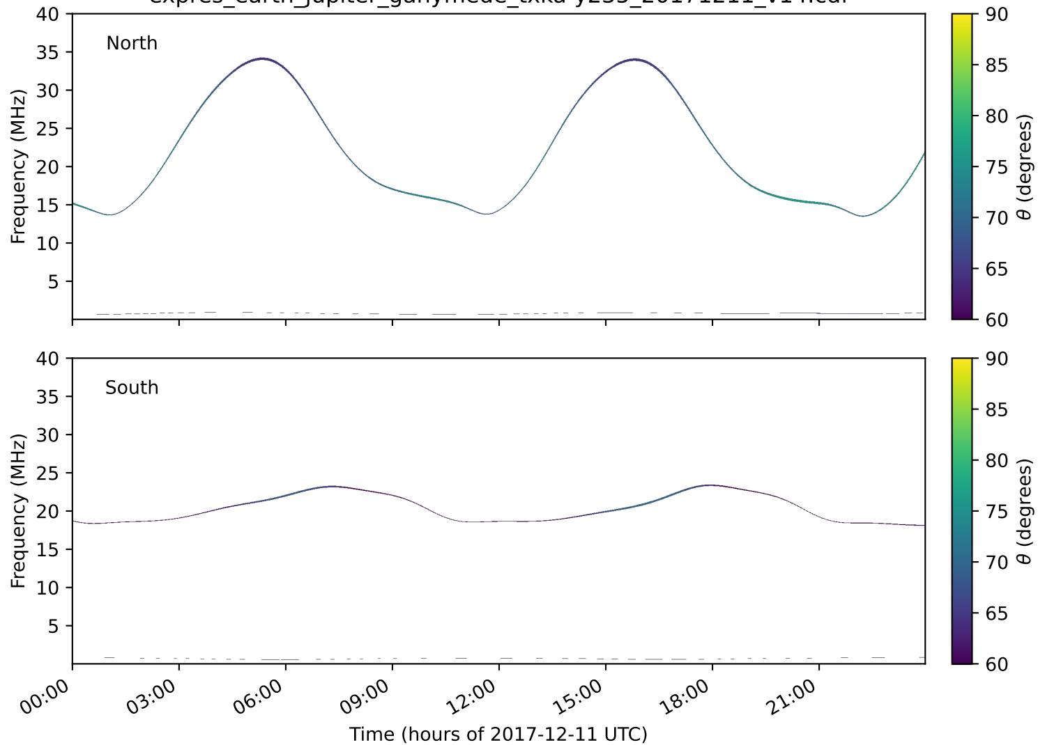
expres_earth_jupiter_ganymede_txka-y235_20171211_v14.cdf
