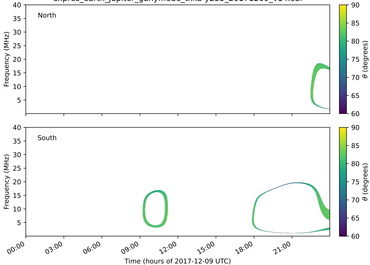
expres_earth_jupiter_ganymede_txka-y235_20171209_v14.cdf
