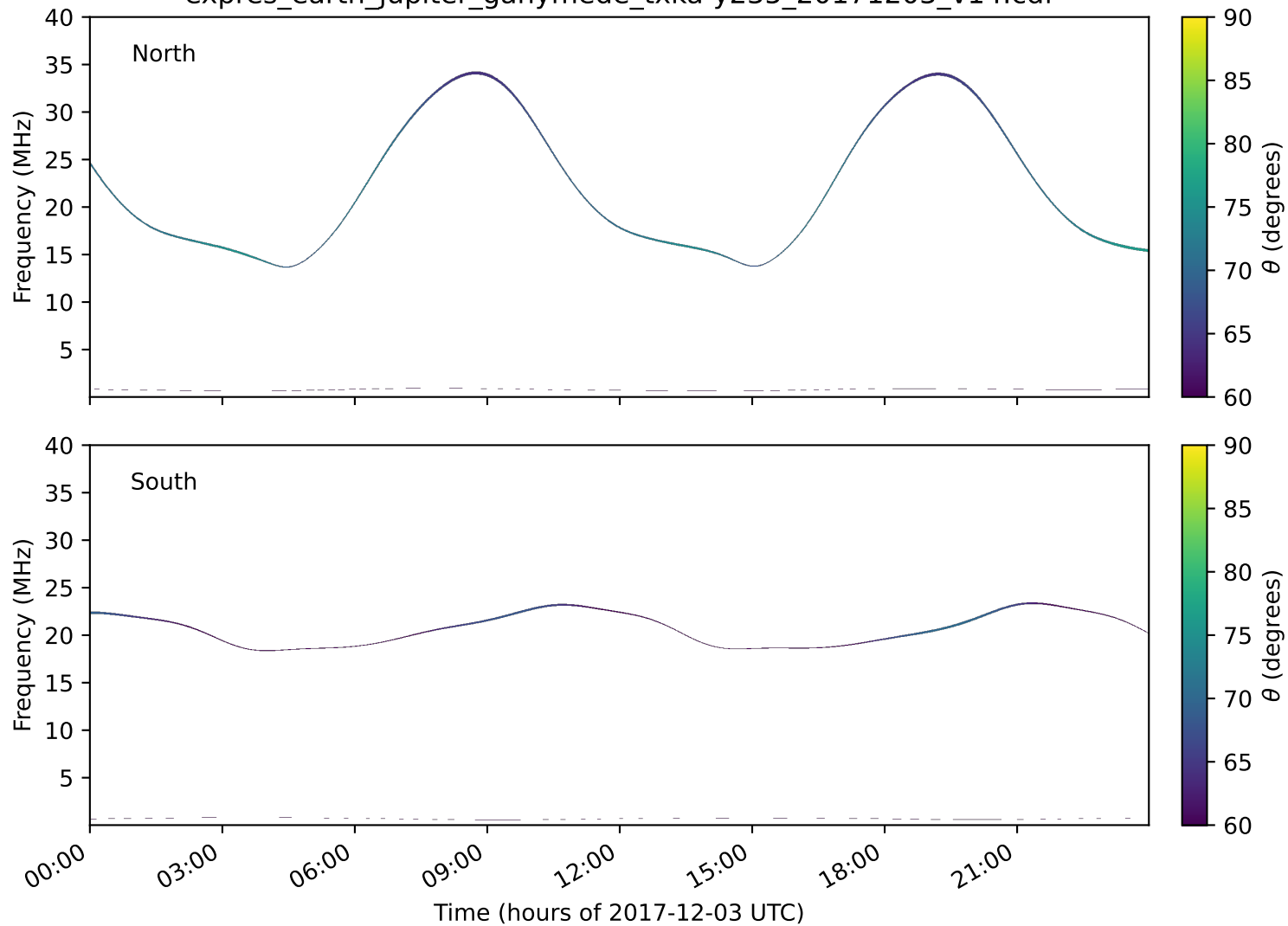
expres_earth_jupiter_ganymede_txka-y235_20171203_v14.cdf
