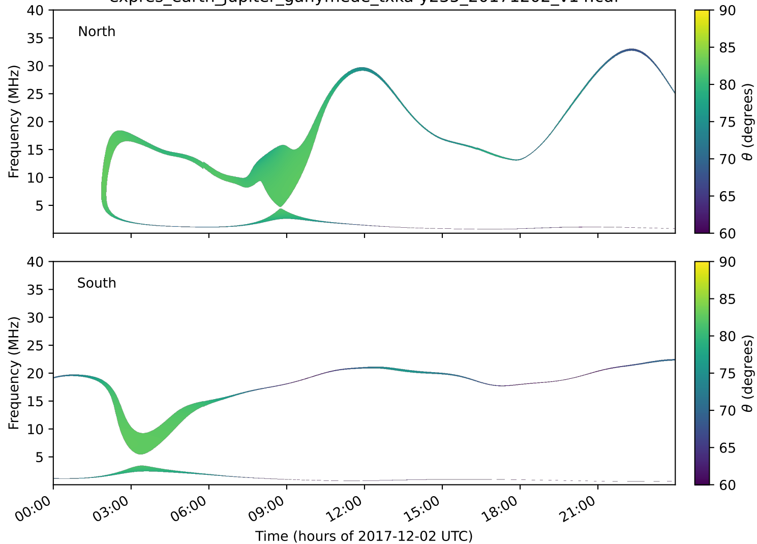
expres_earth_jupiter_ganymede_txka-y235_20171202_v14.cdf
