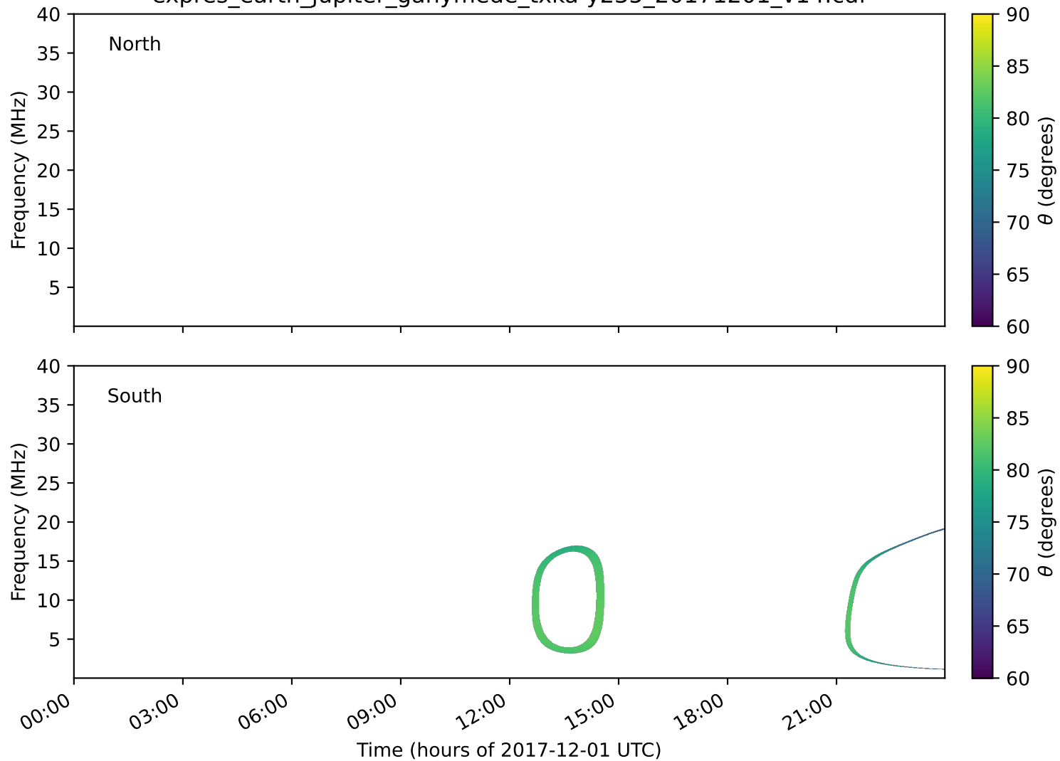
expres_earth_jupiter_ganymede_txka-y235_20171201_v14.cdf
