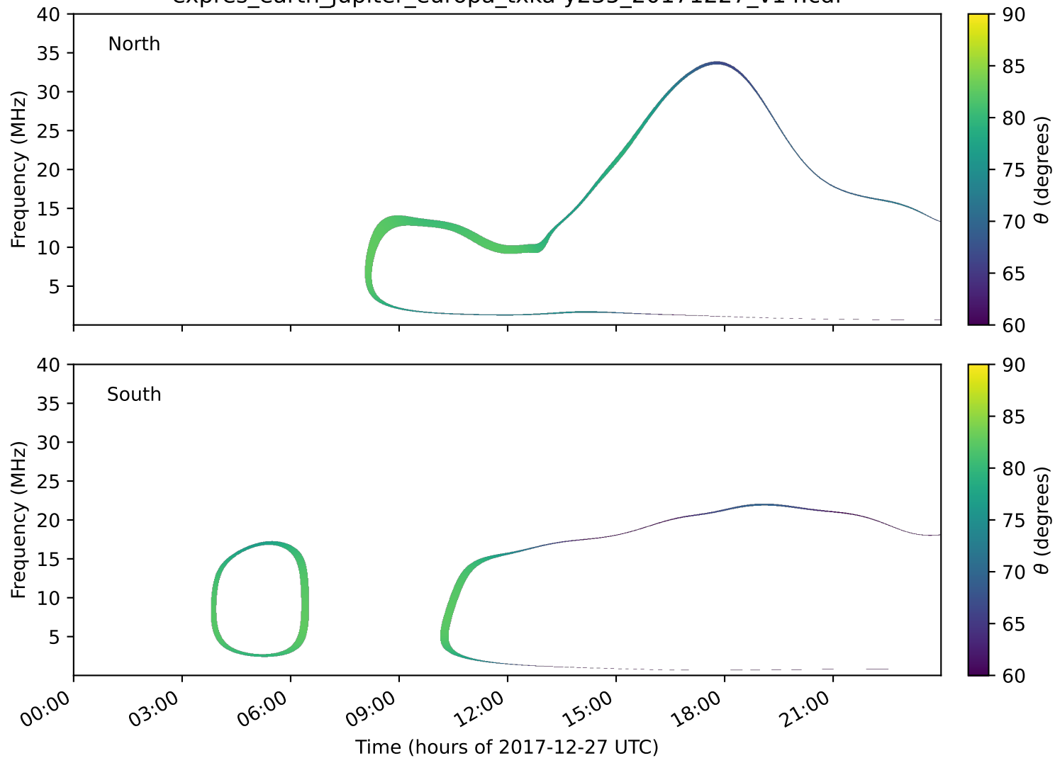
expres_earth_jupiter_europa_txka-y235_20171227_v14.cdf
