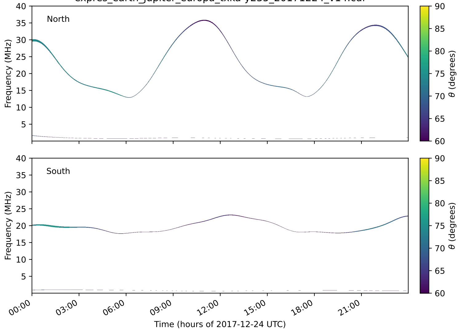
expres_earth_jupiter_europa_txka-y235_20171224_v14.cdf
