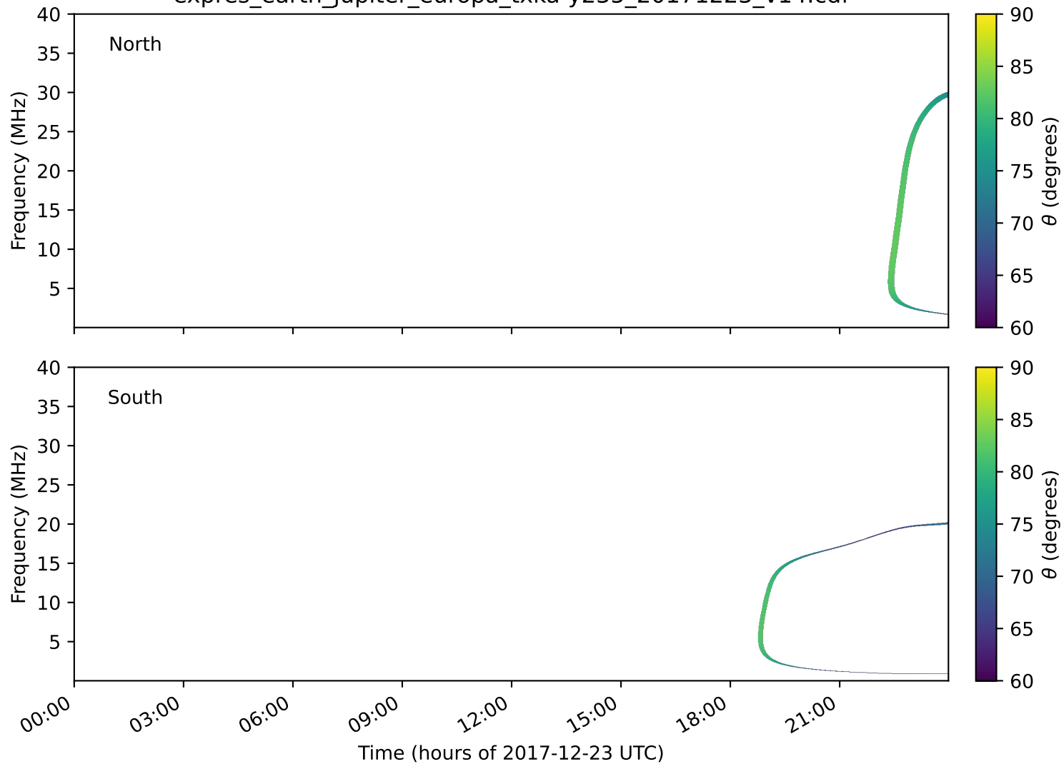
expres_earth_jupiter_europa_txka-y235_20171223_v14.cdf
