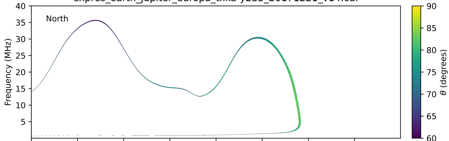
expres_earth_jupiter_europa_txka-y235_20171221_v14.cdf
