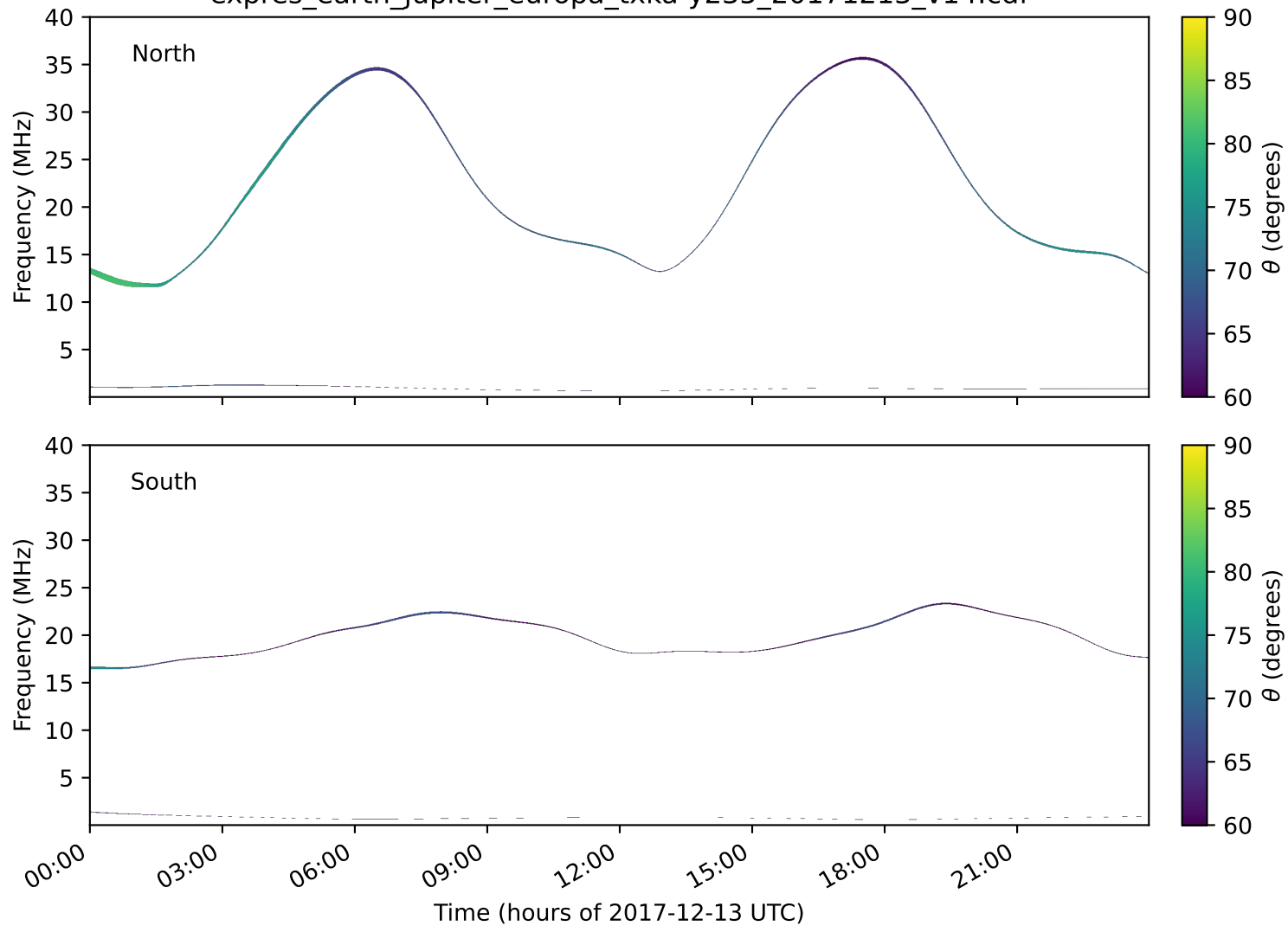
expres_earth_jupiter_europa_txka-y235_20171213_v14.cdf
