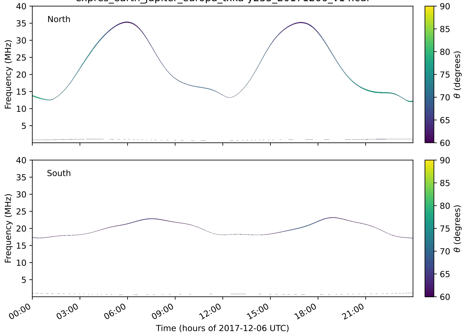
expres_earth_jupiter_europa_txka-y235_20171206_v14.cdf
