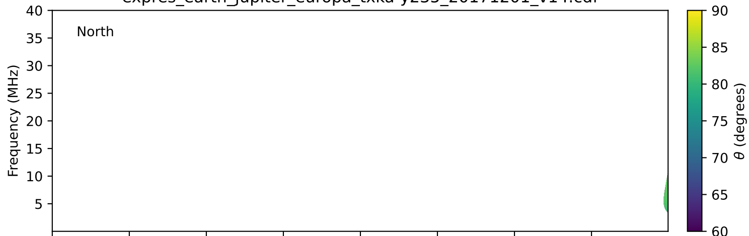
expres_earth_jupiter_europa_txka-y235_20171201_v14.cdf
