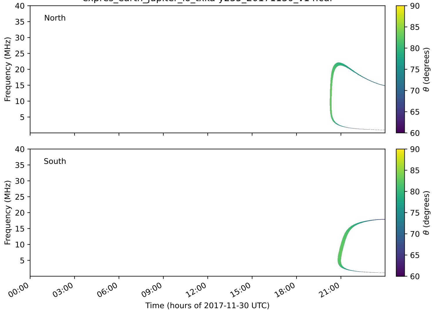
expres_earth_jupiter_io_txka-y235_20171130_v14.cdf
