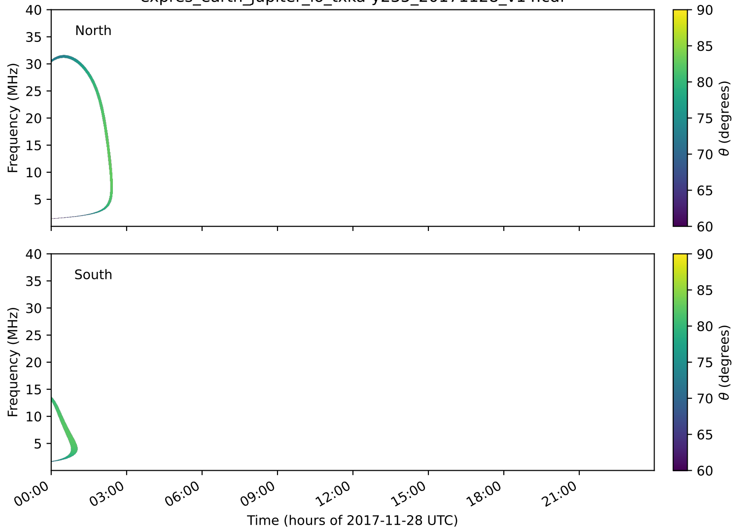
expres_earth_jupiter_io_txka-y235_20171128_v14.cdf
