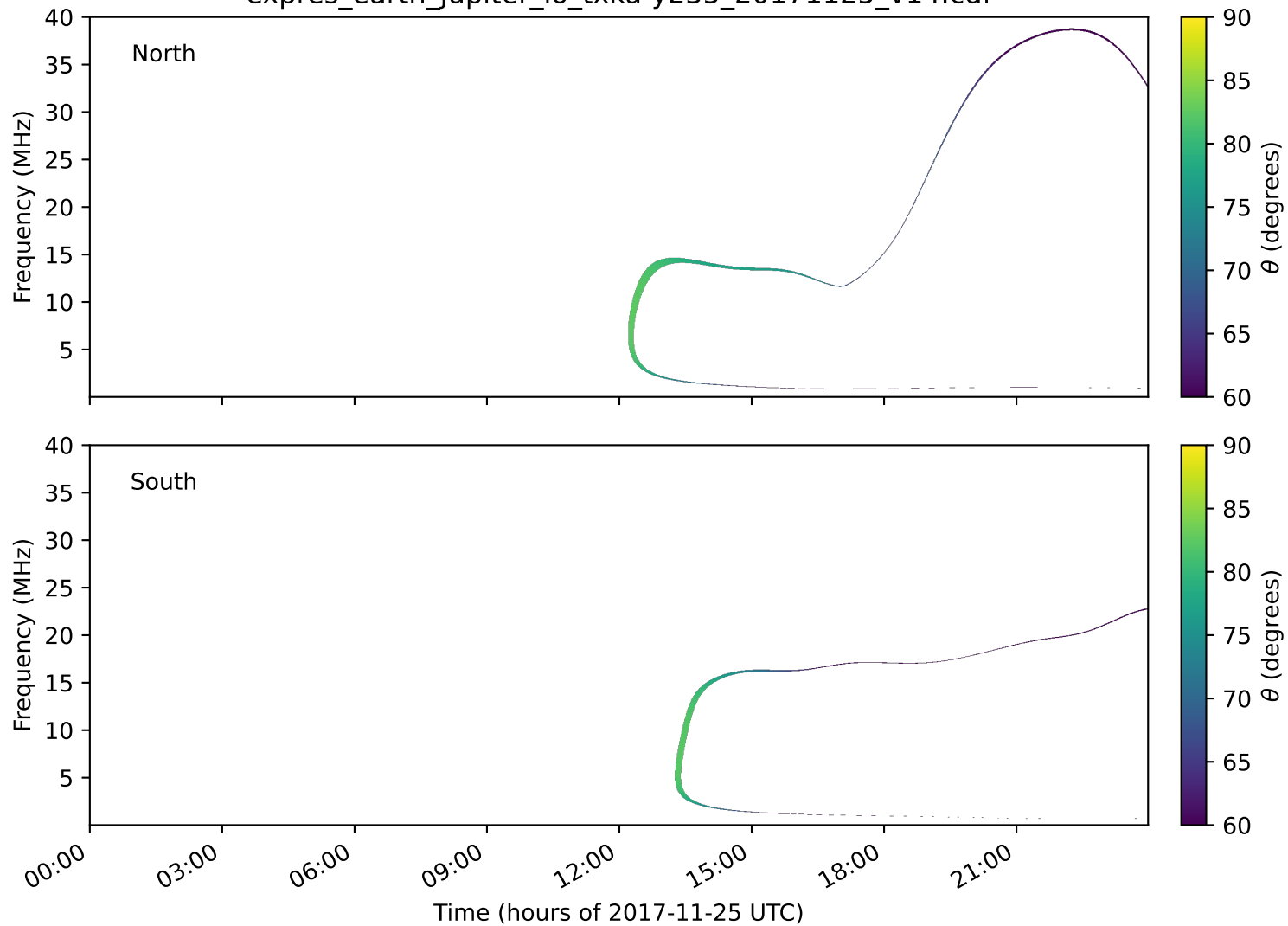
expres_earth_jupiter_io_txka-y235_20171125_v14.cdf
