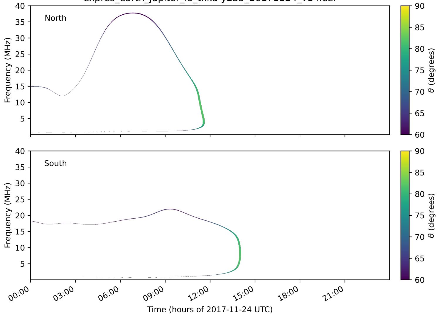
expres_earth_jupiter_io_txka-y235_20171124_v14.cdf
