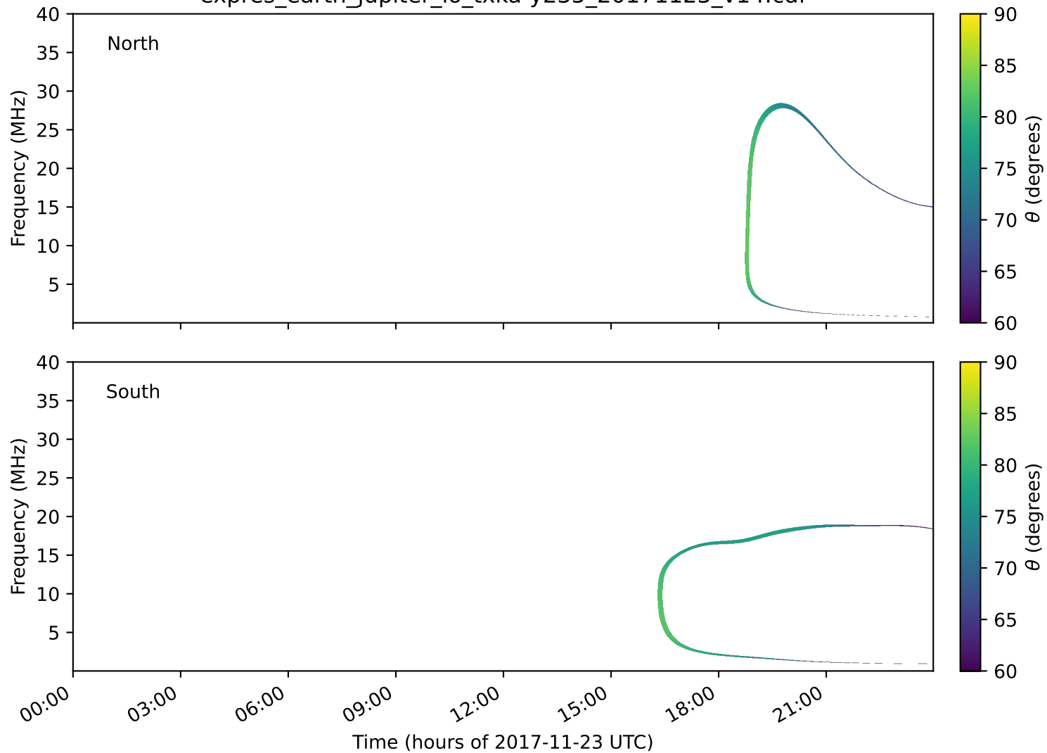
expres_earth_jupiter_io_txka-y235_20171123_v14.cdf
