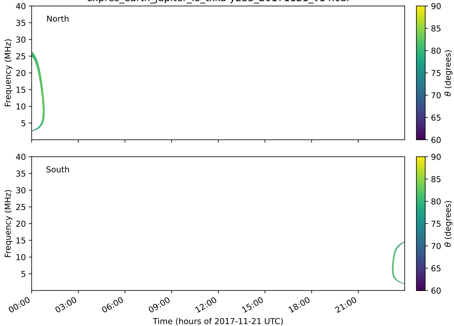
expres_earth_jupiter_io_txka-y235_20171121_v14.cdf
